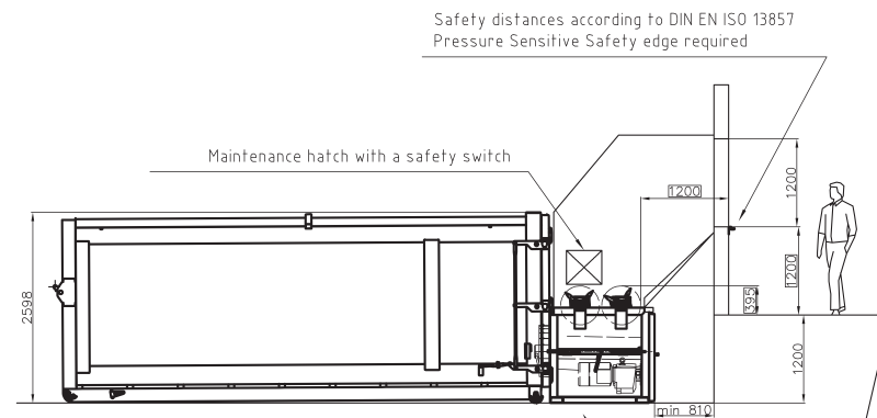
H&G Screw / 31 m 3 container
